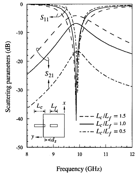
Fig. 6. Calculated frequency responses for the antennas with different coupling aperture lengths L_c . The stub lengths l_f and l_c are, respectively, 1.1 and 4.6 mm for L_c/L_f = 0.5 , 1.3, and 2.9 mm for L_c/L_f = 1.0 , 1.6, and 1.8 mm for L_c/L_f = 1.5 . d_s = 1 mm. The other parameters are the same as those in Fig. 2.
