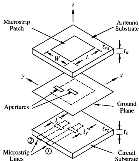
Fig. 1. Geometry of a two-port aperture-coupled microstrip antenna.
